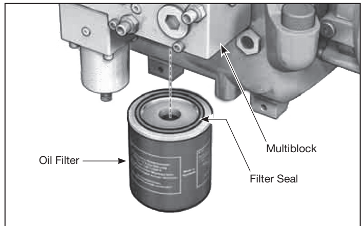
Figure 12 - Oil Filter
