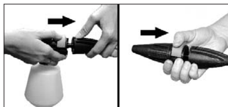
Figure 7- Attach nozzle to lance or detergent bottle
