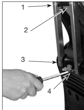
Figure 4 -Attach phillips screws (PW182501 only)
