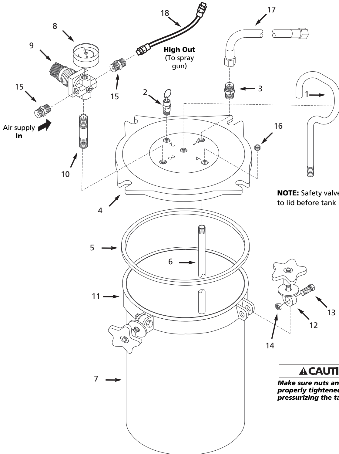
Figure 7 — Repair Parts Illustration
