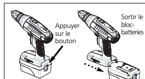
Figure 2 Retirer le bloc-batteries – DG111200CD, DG111400CD, DG111900CD and DG151900CD
