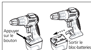
Figure 1 Retirer le bloc-batteries – DG100600CD, DG110400CD and DG110600CD
