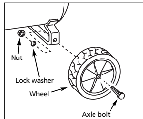
Figure 2 - Wheel Assembly
