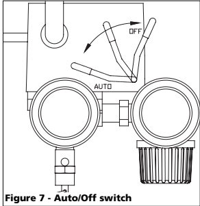
Figure 7 - Auto/Off switch
