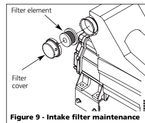
Figure 9 - Intake filter maintenance
