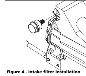
Figure 4 - Intake filter installation
