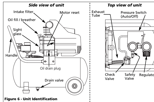
Figure 6 - Unit Identification
