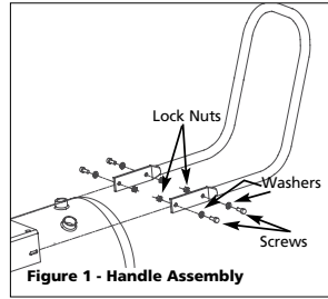
Figure 1 - Handle Assembly
