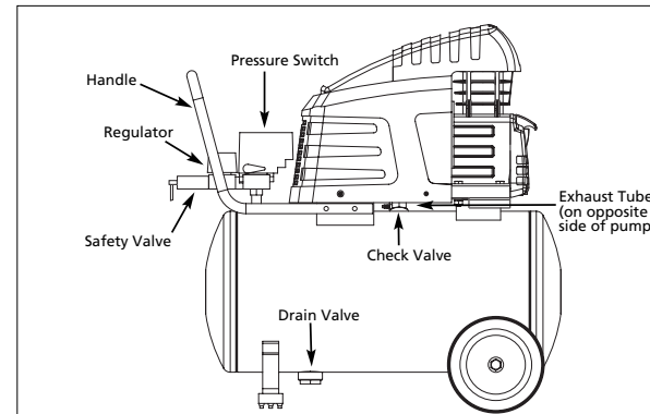
Figure 5 - Unit Identification
