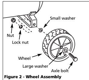
Figure 2 - Wheel Assembly
